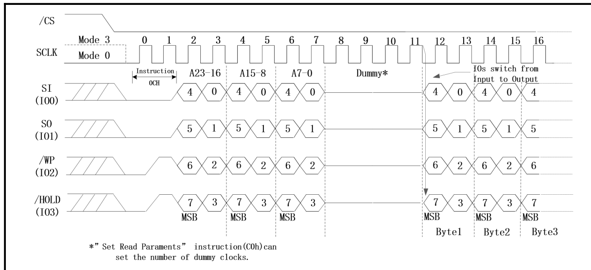
Figure 36. Burst Read with Wrap (QPI Mode only)
