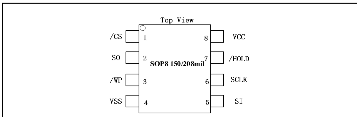
Figure 2. Pin Configuration SOP8 150mil/208 mil
