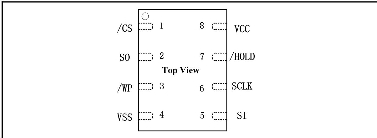
Figure 3. Pin Configuration WSON8 5X6mm and USON8 4X4mm
