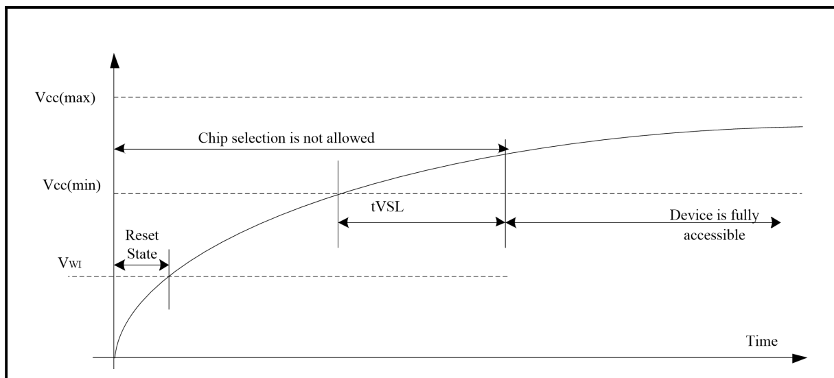
Figure 72. Power-up Timing and Voltage Levels
