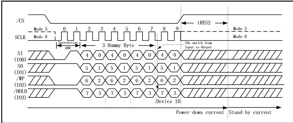
Figure 49. Release Power-Down/Read Device ID Sequence Diagram (QPI Mode)
