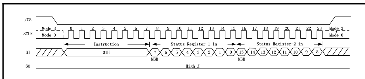
Figure 13. Write Status Register Sequence Diagram-01H 2byte (SPI Mode)
