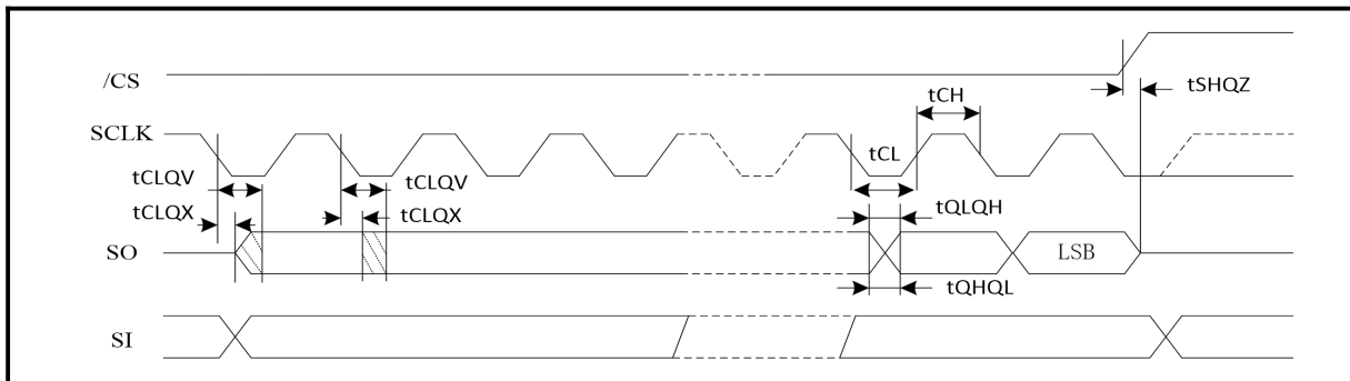
Figure 76. Hold Timing
