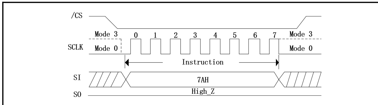
Figure 71. Program/Erase Resume Instruction Sequence (SPI Mode)
