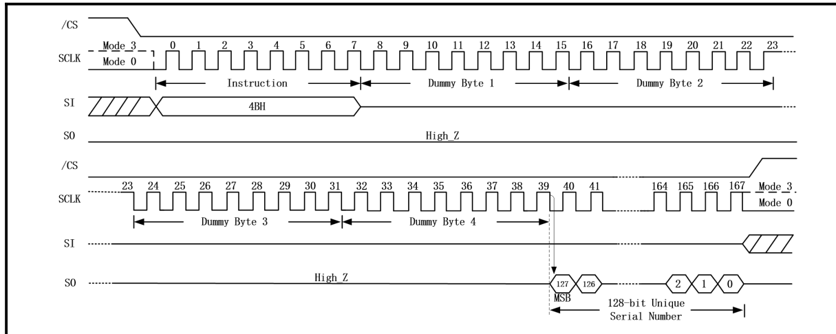
Figure 43. Read Unique ID Sequence Diagram (SPI Mode only)
