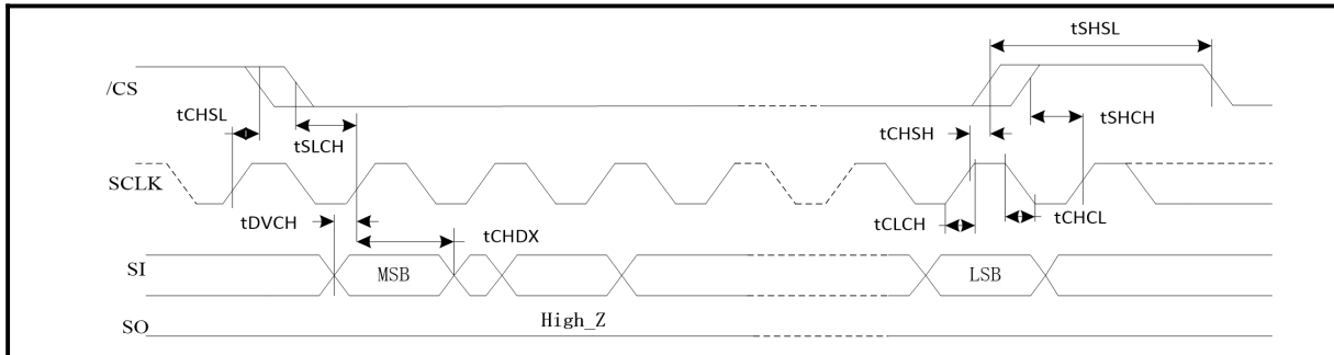
Figure 75. Output Timing
