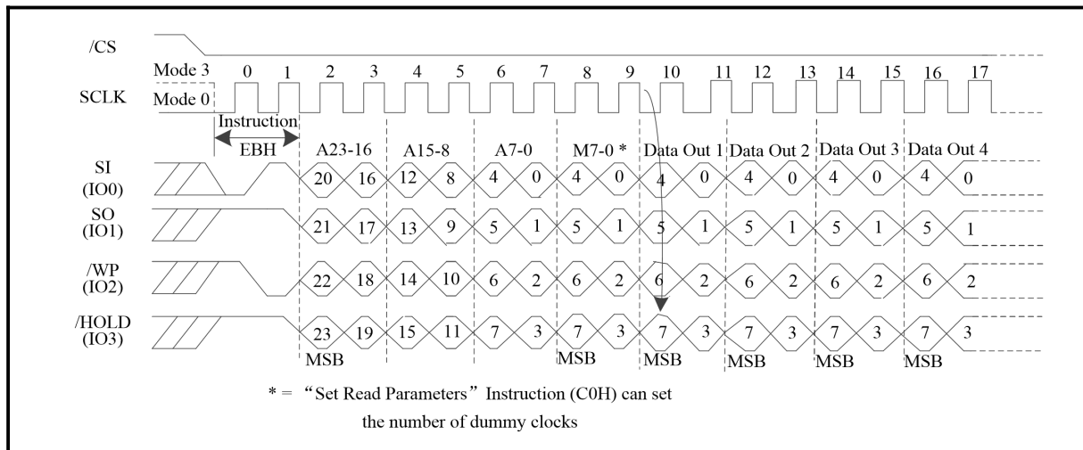
Figure 32. Quad I/O Fast Read Sequence Diagram (QPI Mode Mode; Initial instruction or previous (M5-4=(1,0)))
