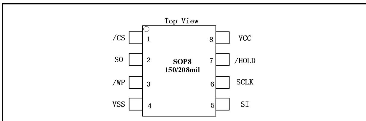
Figure 2. Pin Configuration SOP 150/208 mil
