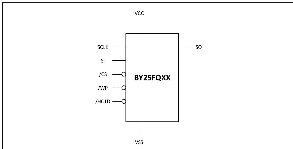
Figure 2. Pin Configuration SOP 150/208 mil
