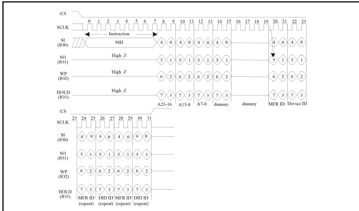
Figure 41. Quad I/O Read Manufacture ID/ Device ID Sequence Diagram (SPI Mode)
