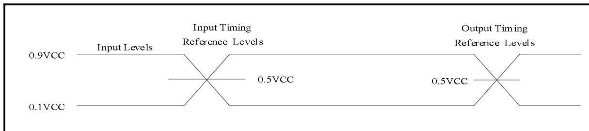
Figure 74. AC Measurement I/O Waveform
