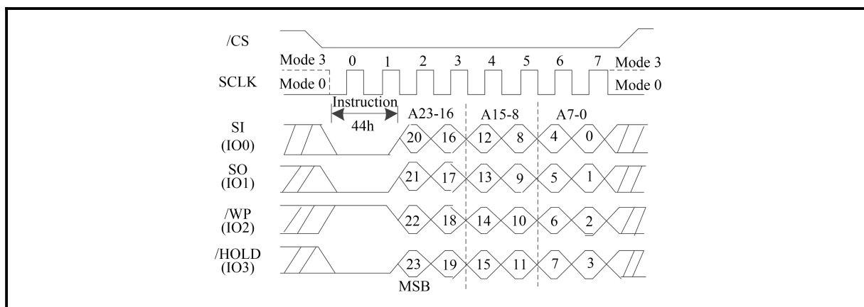
Figure 54. Erase Security Registers instruction Sequence Diagram (QPI Mode)
