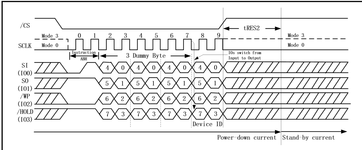
Figure 50. Release Power-Down/Read Device ID Sequence Diagram (QPI Mode)
