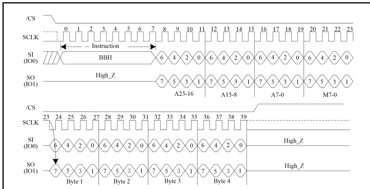
Figure 27. Dual I/O Fast Read Sequence Diagram (Initial instruction or previous (M5-4) ≠ (1,0) , SPI Mode only)
