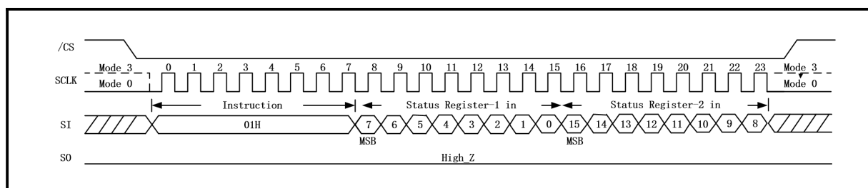
Figure 14. Write Status Register Sequence Diagram-01H 2byte (SPI Mode)
