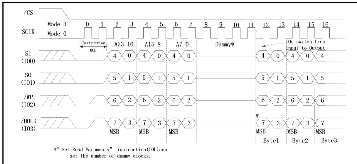
Figure 37. Burst Read with Wrap (QPI Mode only)
