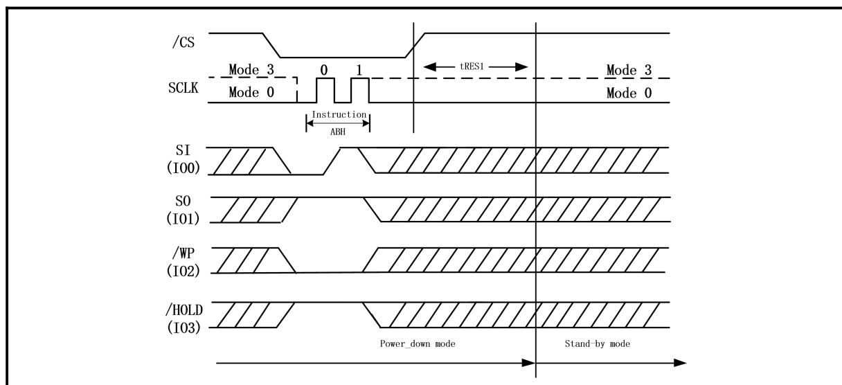
Figure 48. Release Power-Down Sequence Diagram (QPI Mode)
