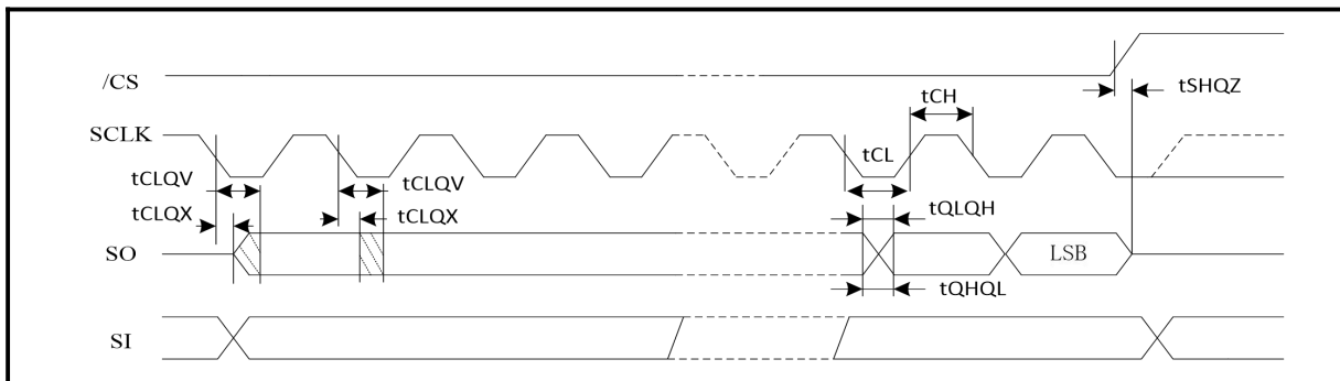
Figure 77. Hold Timing
