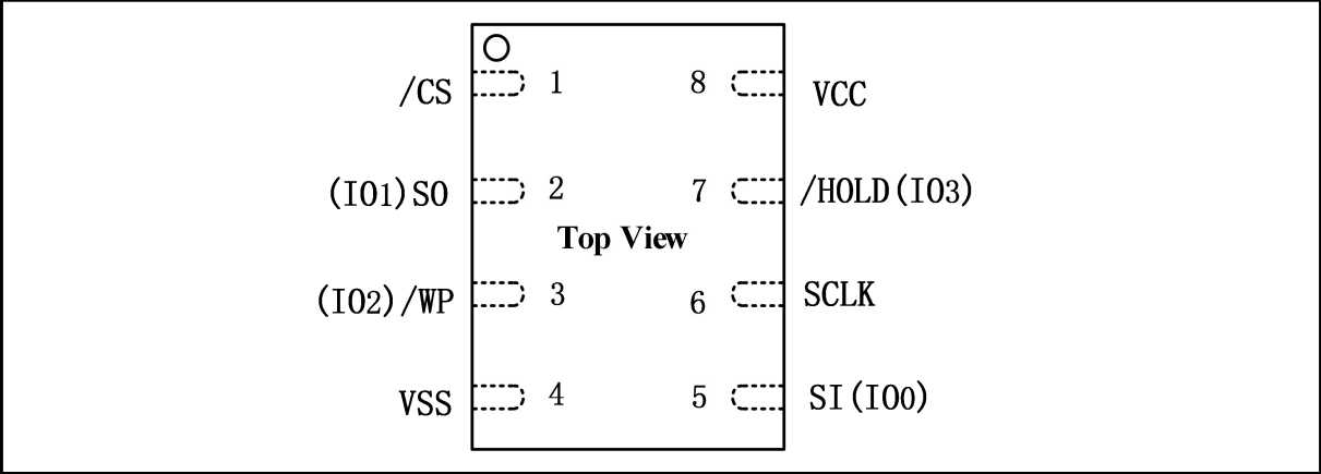
Figure 3. Pin Configuration WSON 5x6-mm and USON 4*3-mm
