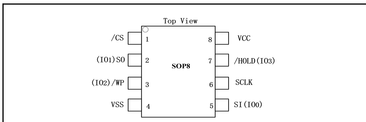
Figure 2. Pin Configuration SOP 150/208 mil
